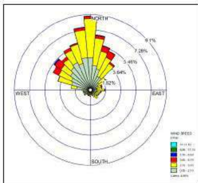
Figure 5.3: Windrose of the study area during November-December 2019 (wind direction blowing towards the centre)
