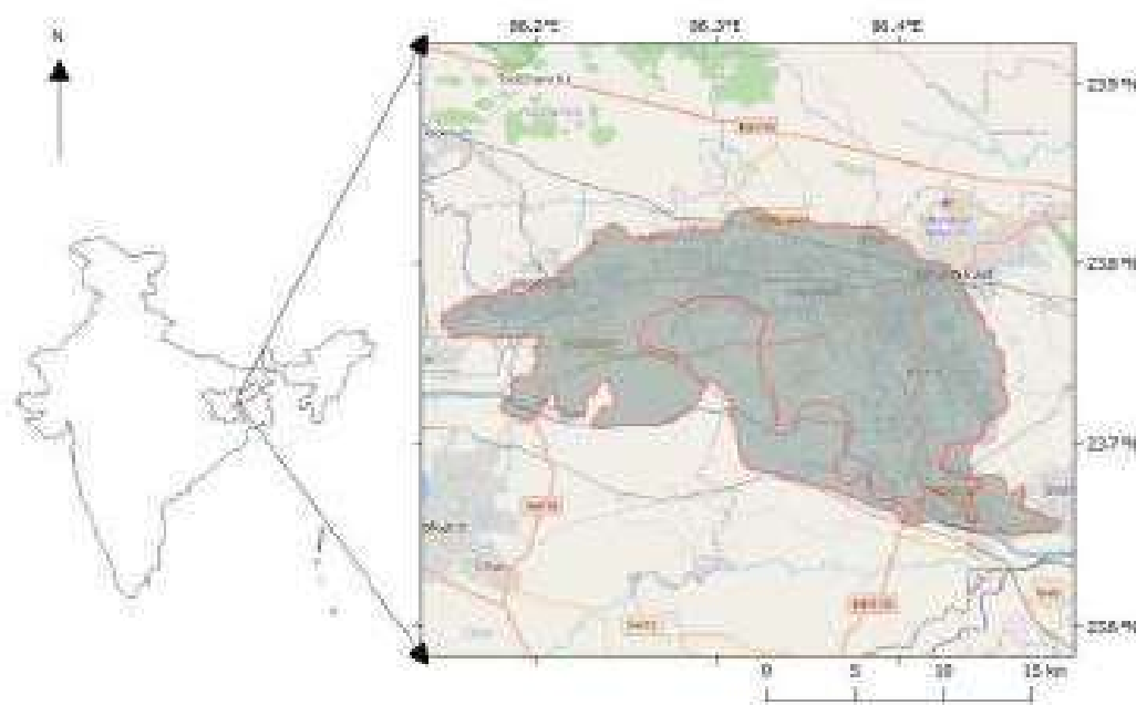
Figure 1.1: Geographical location of Jharia Coalfield in India
