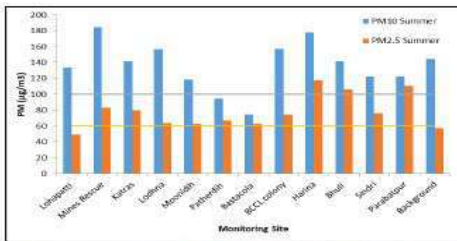
Figure 3.2: Average concentration of PM 10 and PM 2.5 in JCF region in summer compared to NAAQS (2009)
