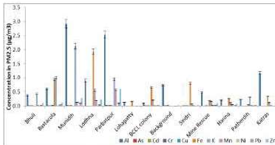
Figure 3.7: Metal concentration of PM 2.5 in winter season
