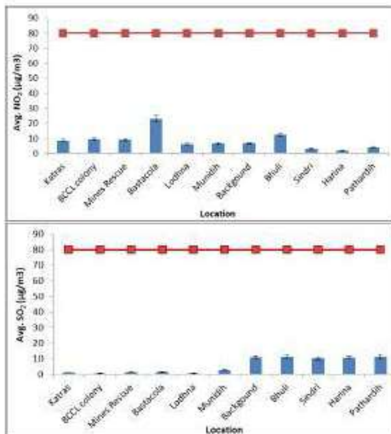
Figure 3.9: NO 2 and SO 2 Concentration of all monitoring sites in Winter season
