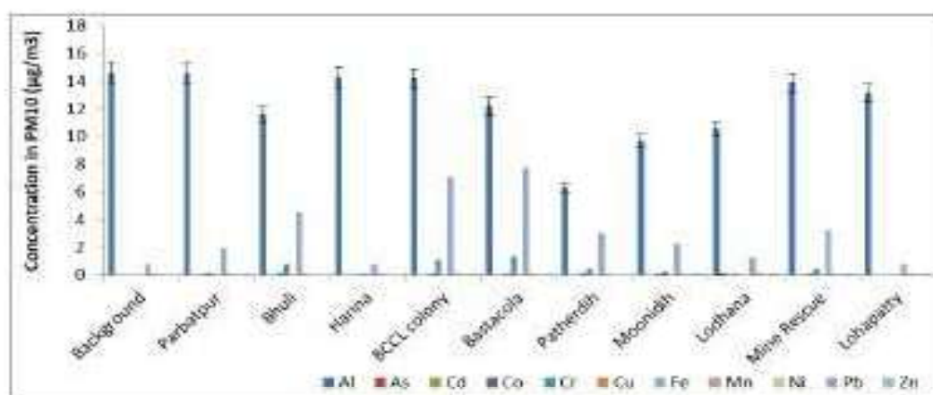
Figure 3.4: Metal concentration of PM 10 in the summer season
