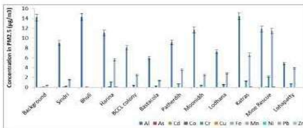
Figure 3.5: Metal concentration of PM 2.5 in the summer season
