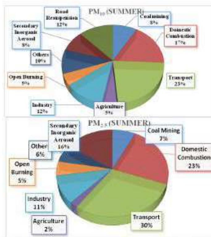
Figure 4.2: Source contribution at receptor locations of PM 10 and PM 2.5 in summer
