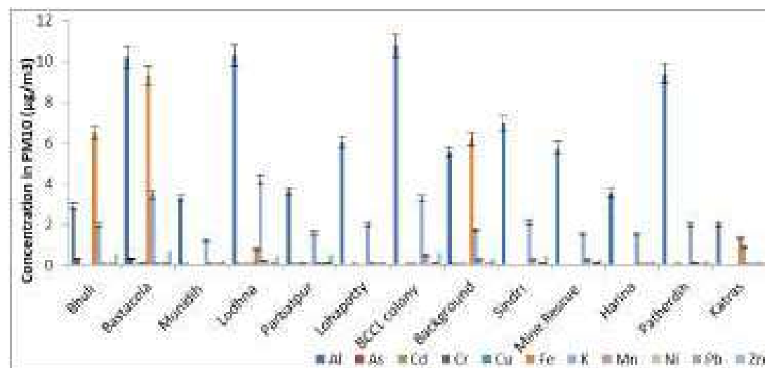
Figure 3.6: Metal concentration of PM 10 in winter season
