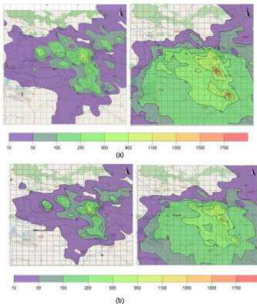
Figure 5.6: 24-hour average maximum ground level concentration of PM contours in the study area simulated during the study periods in summer (left) and winter (right) seasons (a) PM 10 ( \mu\text{g}/\text{m}^3 ) and (b) PM 2.5 ( \mu\text{g}/\text{m}^3 )
