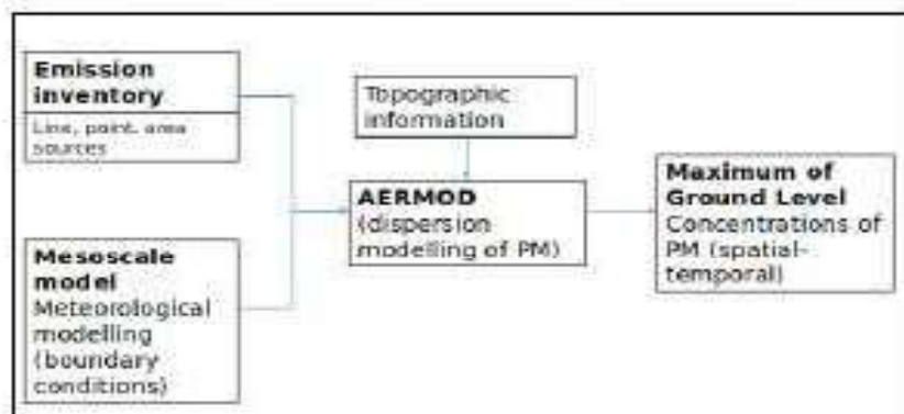
Figure 5.1: Methodology followed in the study.
